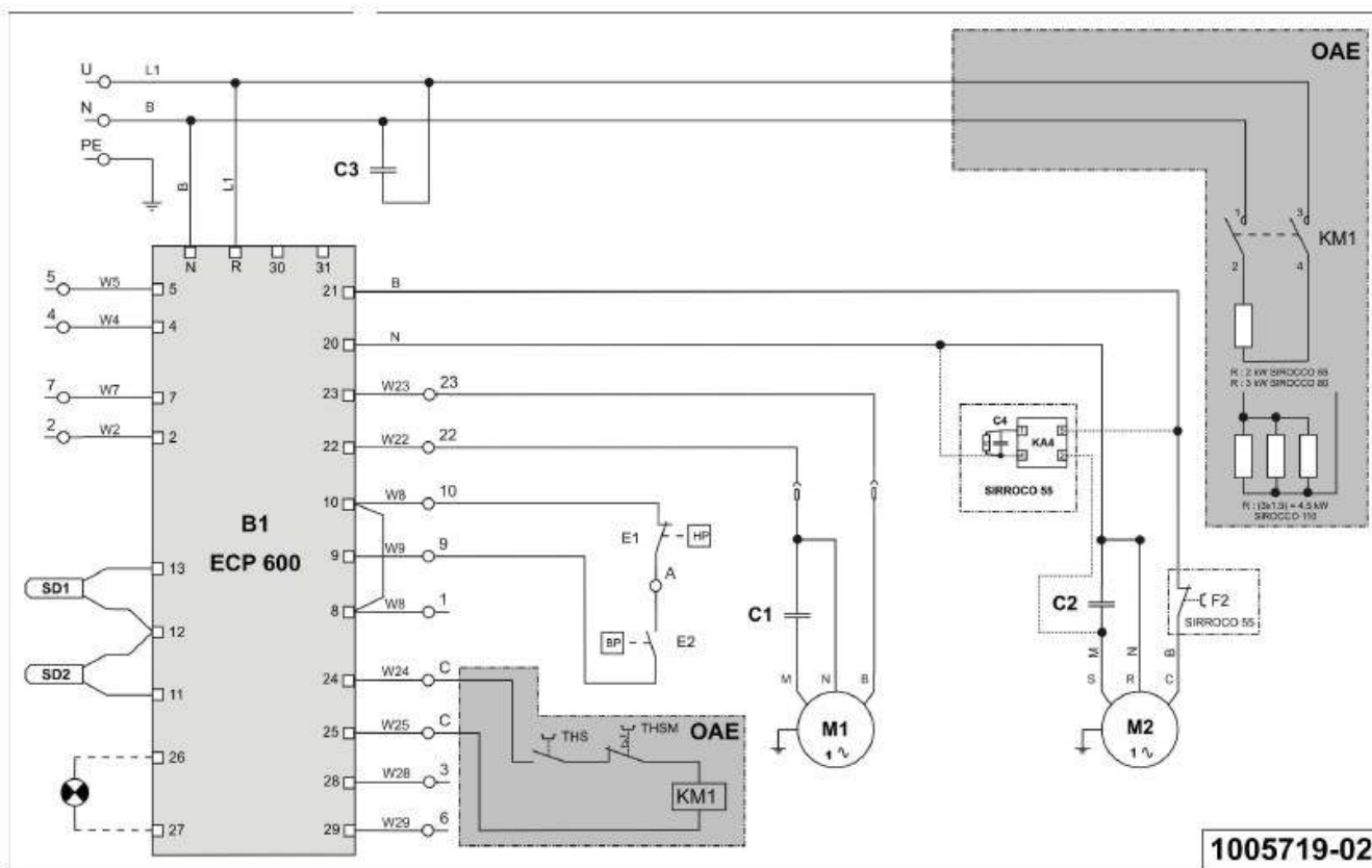
Electric diagram
